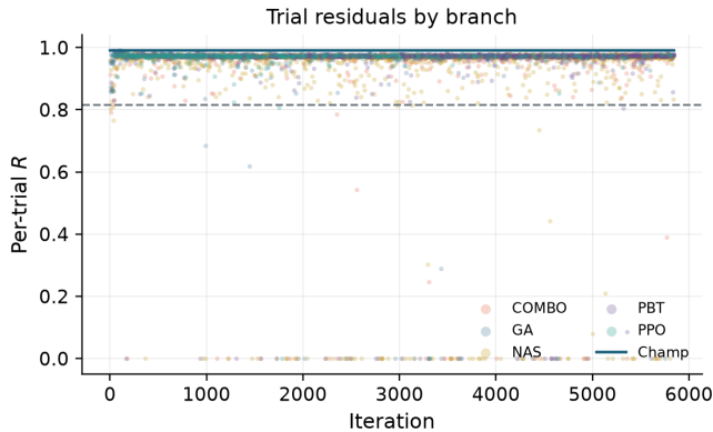
Figure 11: Per-trial residual scatter by search branch at the 5k-gate freeze, with champion overlay.
