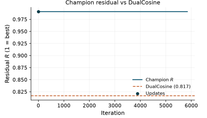
Figure 8: Overnight 5k-gate freeze: champion residual R versus clean search iteration, with DualCosine baseline on the runner geometry (RTX 3090).
