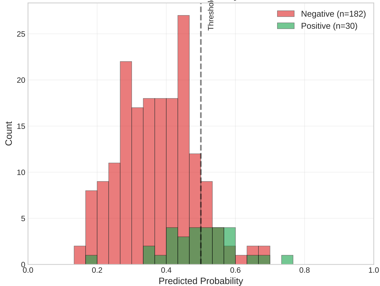
Score Distribution by Class
