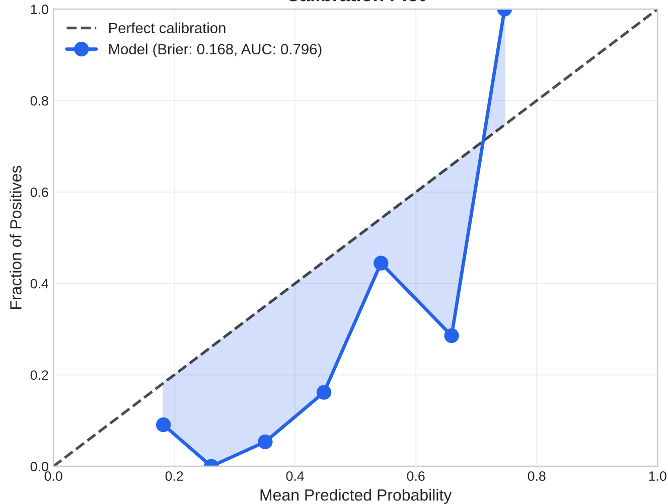
Calibration Plot
