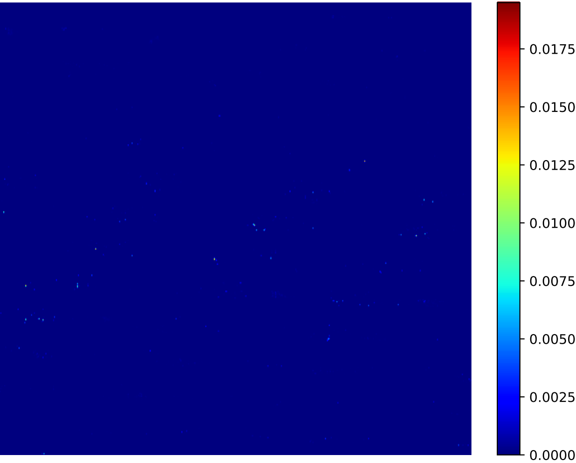
Attention Heatmap - 15
