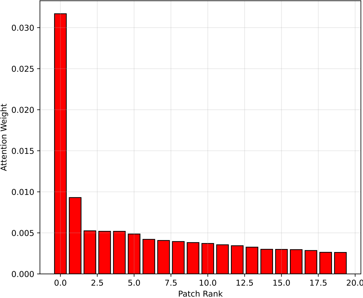
Top-20 Patches Cumulative: 0.109
