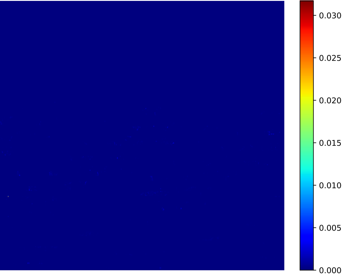
Attention Heatmap - 185
