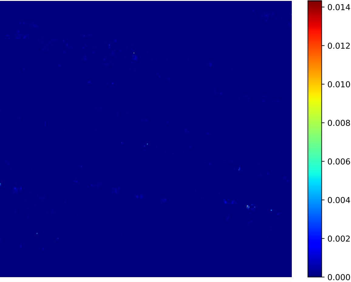
Attention Heatmap - 186
