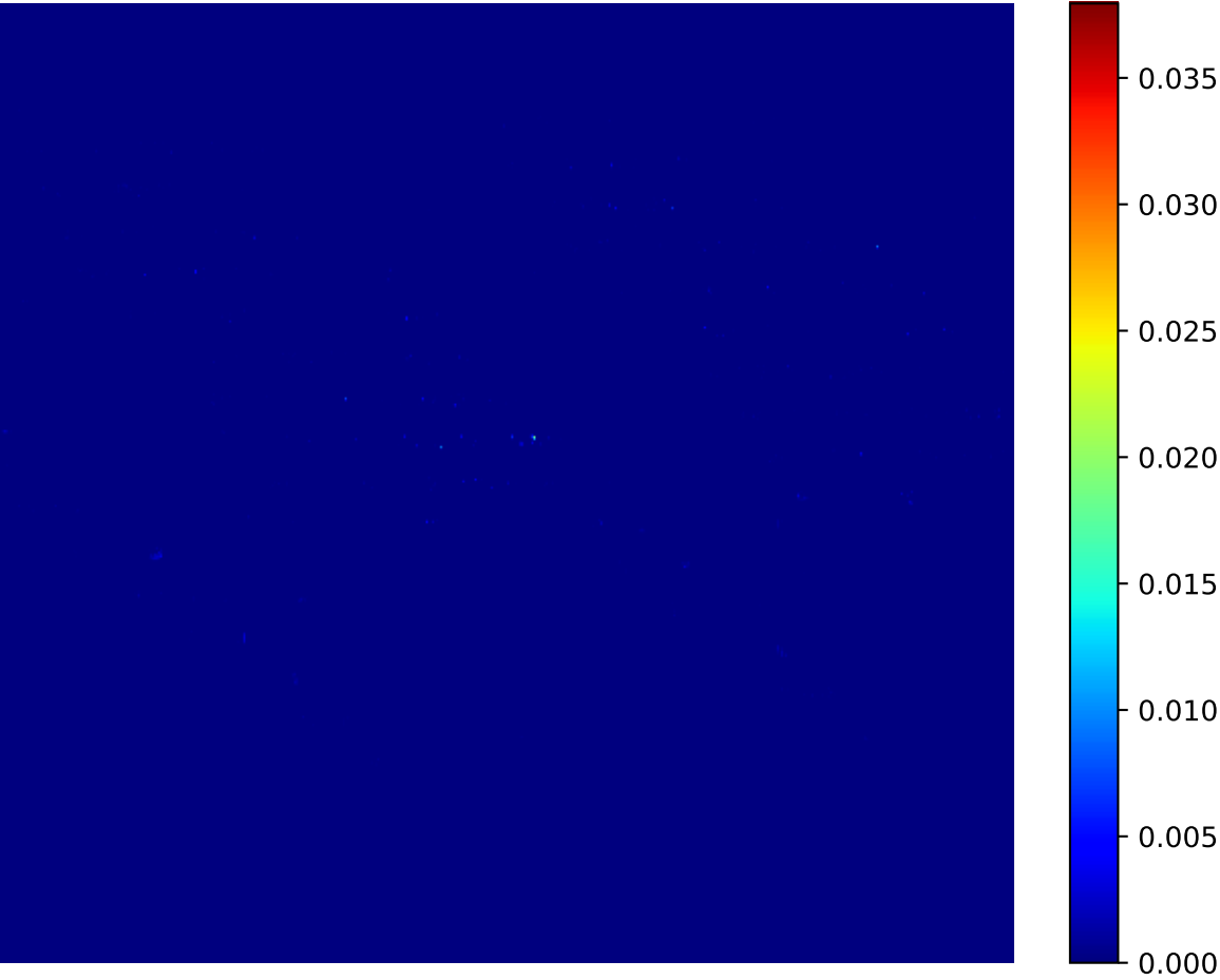
Attention Heatmap - 187
