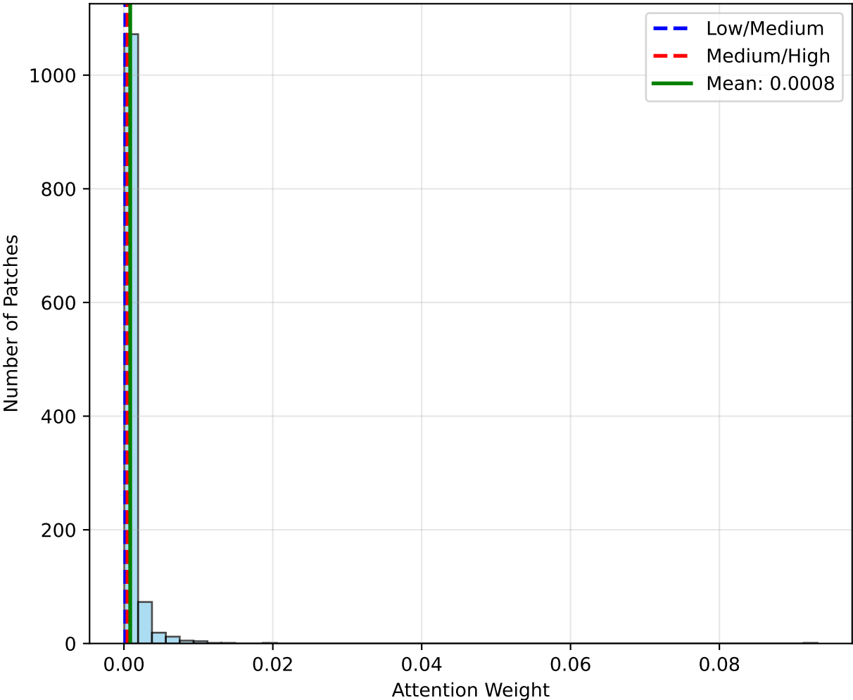
Attention Distribution Entropy: 5.939
