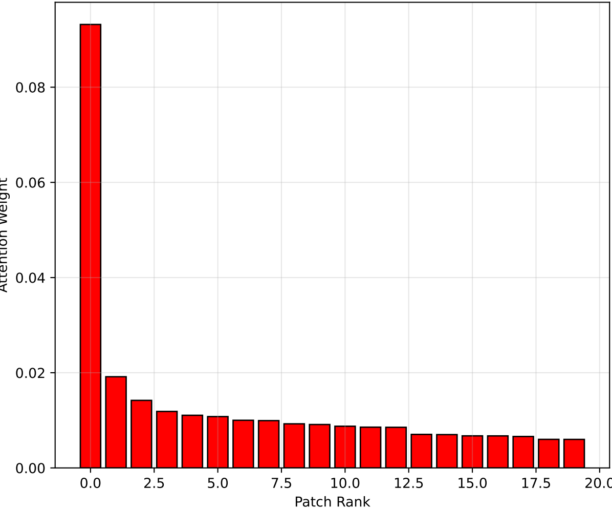
Top-20 Patches Cumulative: 0.271
