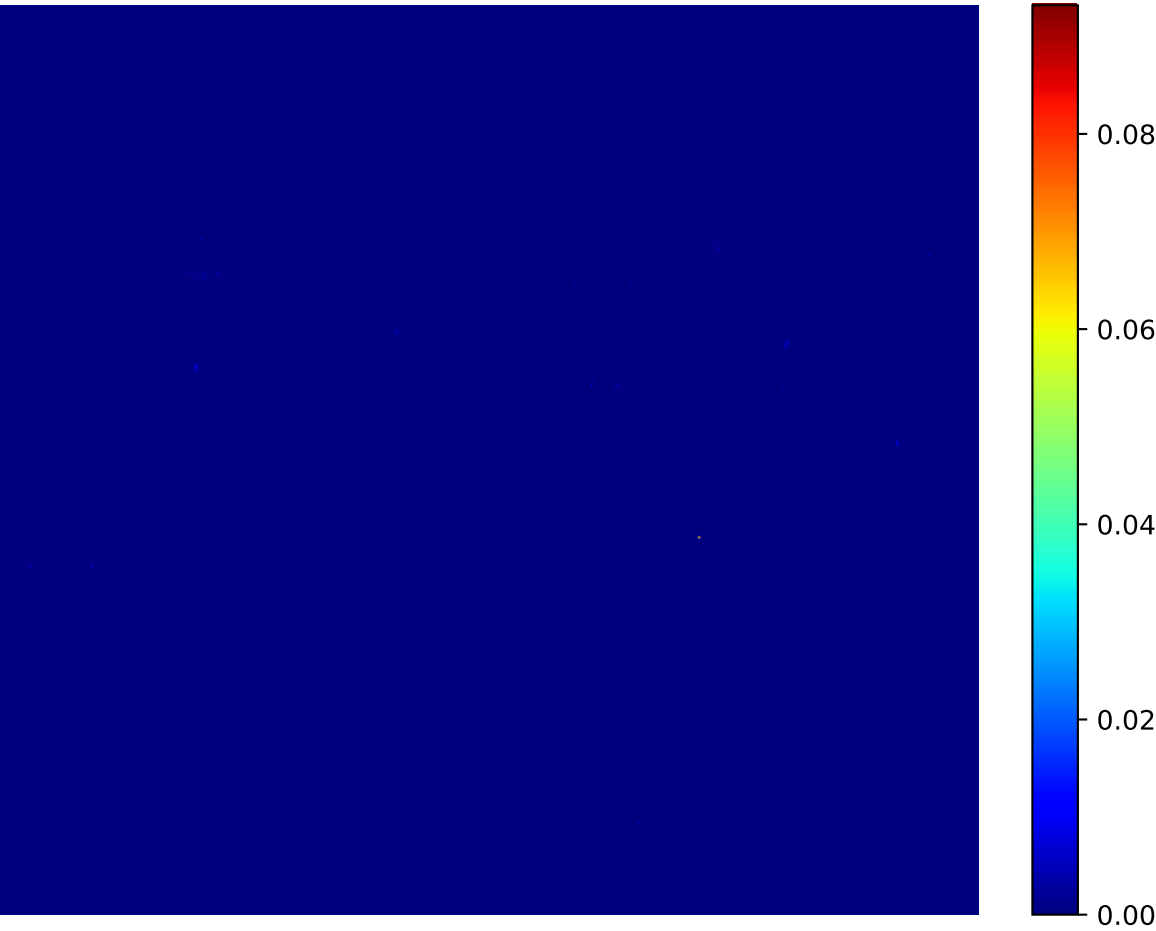
Attention Heatmap - 188
