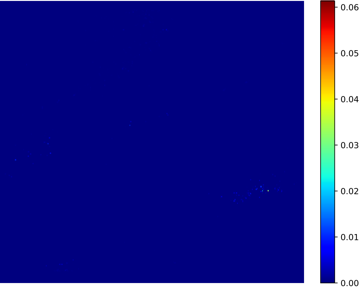
Attention Heatmap - 194
