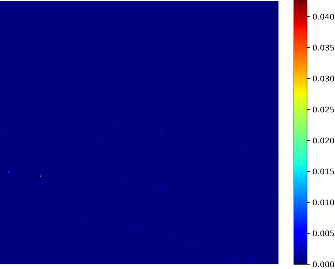
Attention Heatmap - 195
