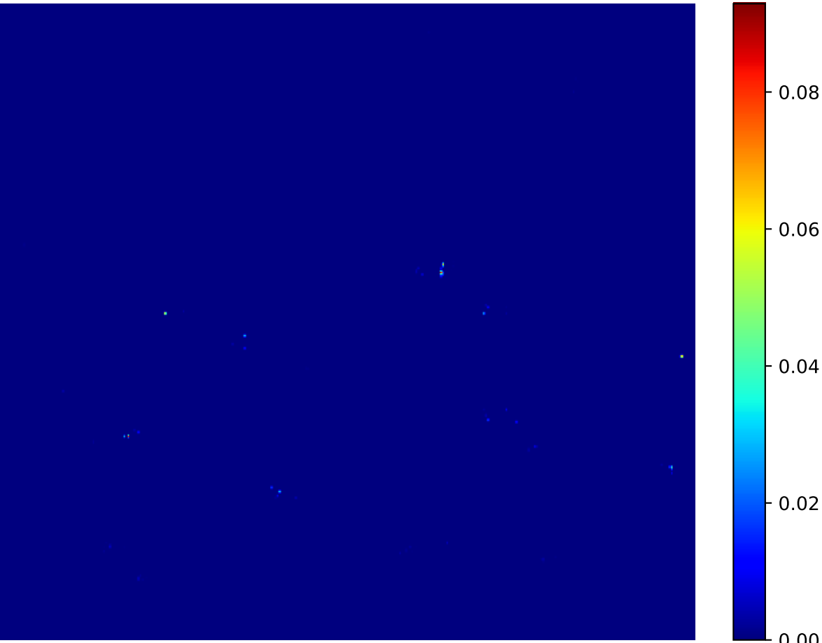
Attention Heatmap - 17
