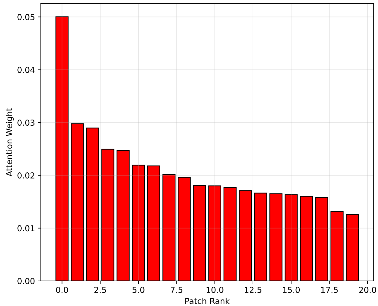
Top-20 Patches Cumulative: 0.420
