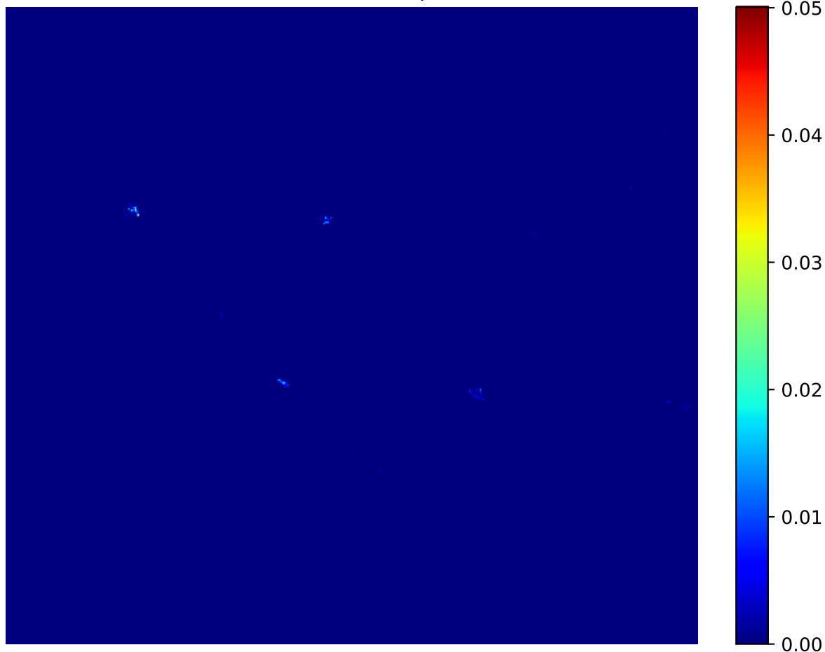
Attention Heatmap - 18
