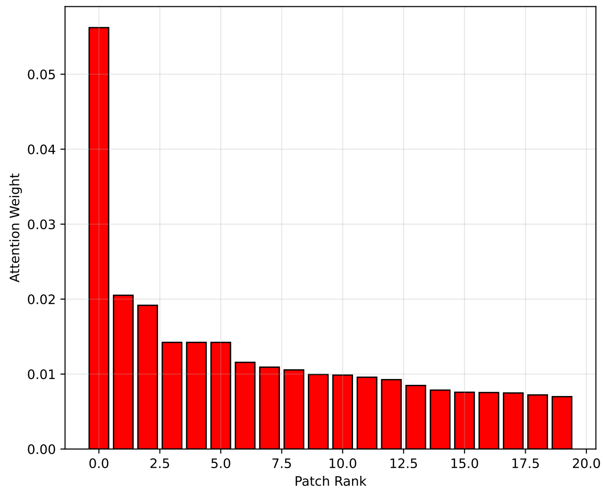
Top-20 Patches Cumulative: 0.263
