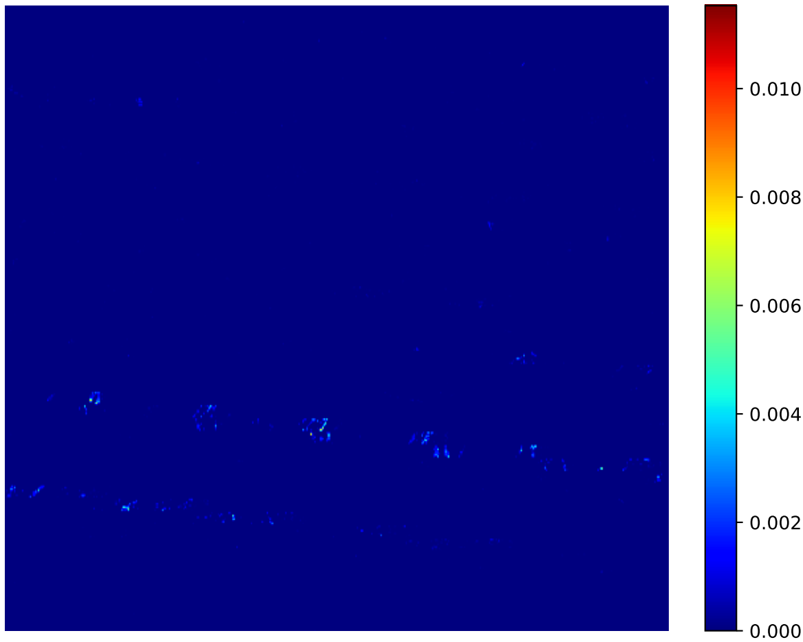
Attention Heatmap - 218
