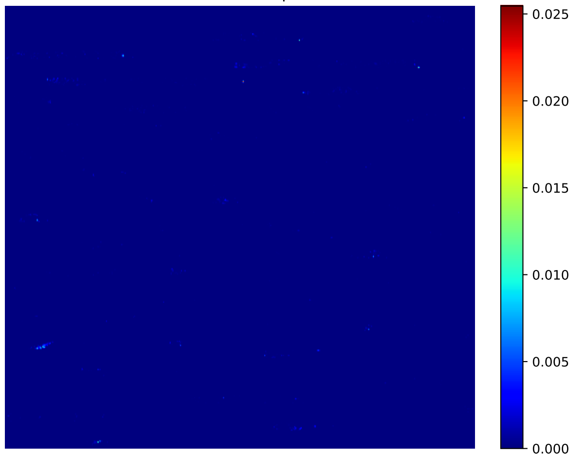
Attention Heatmap - 246
