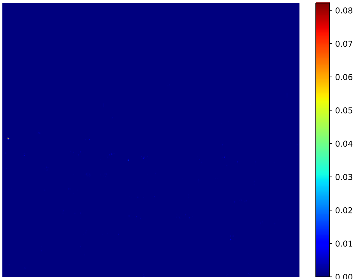
Attention Heatmap - 248
