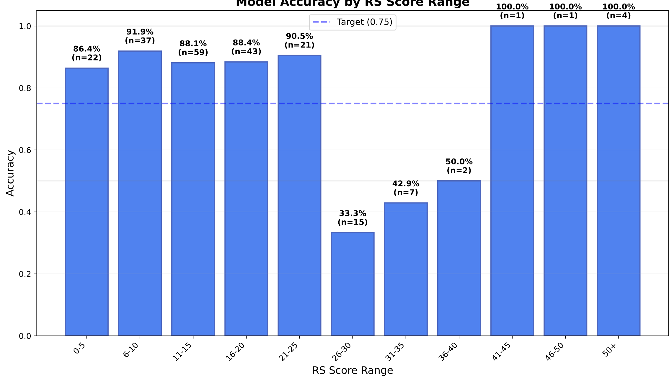
Model Accuracy by RS Score Range
