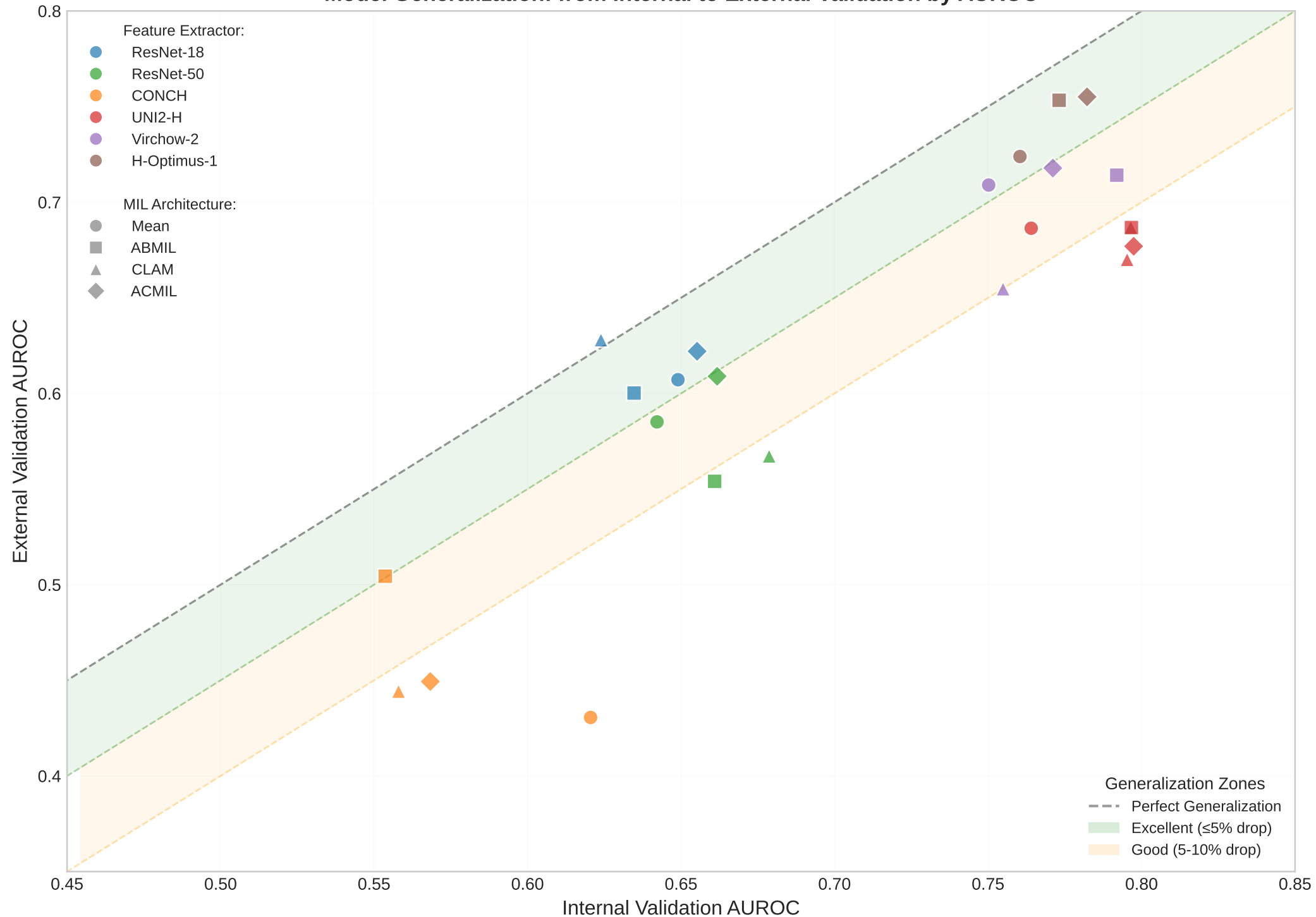
Model Generalization: from Internal to External Validation by AUROC
