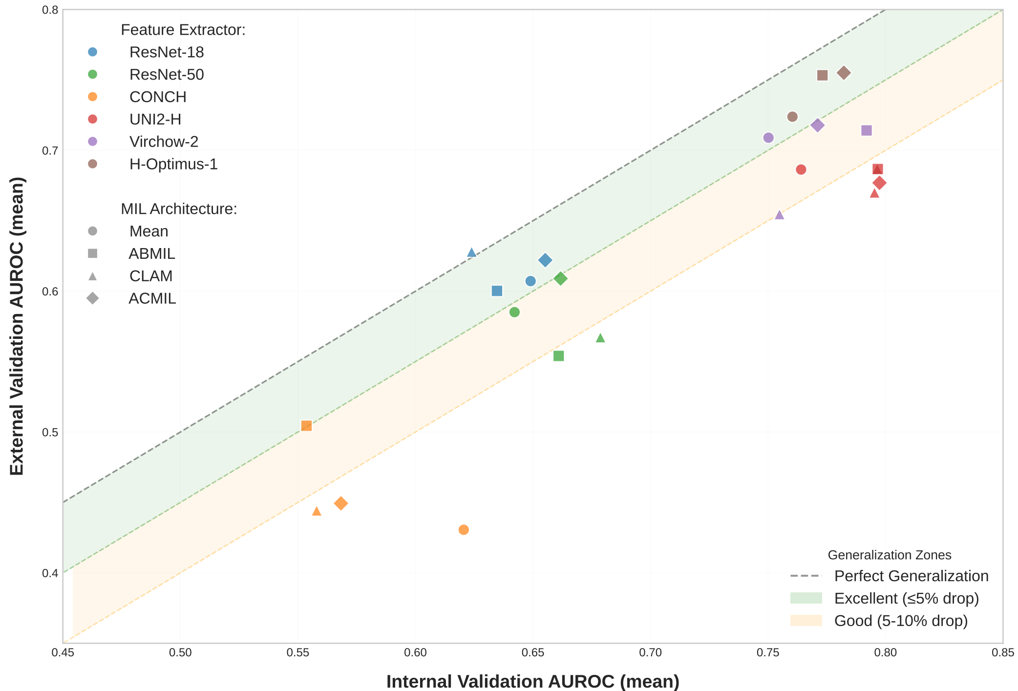
Model Generalization Performance
