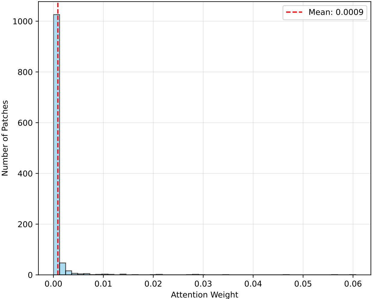
Attention Distribution Entropy: 5.251
