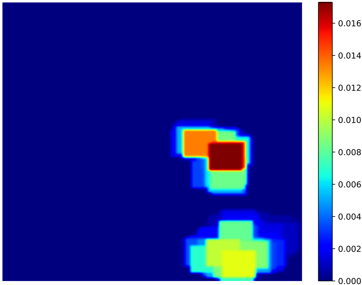
Attention Heatmap - 47
