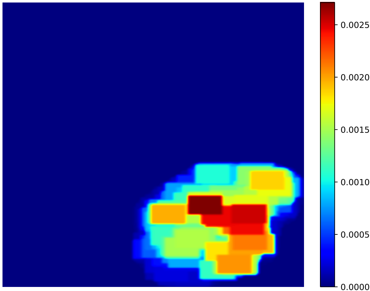
Attention Heatmap - 76
