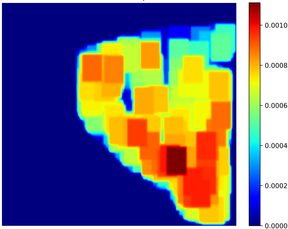
Attention Heatmap - 63
