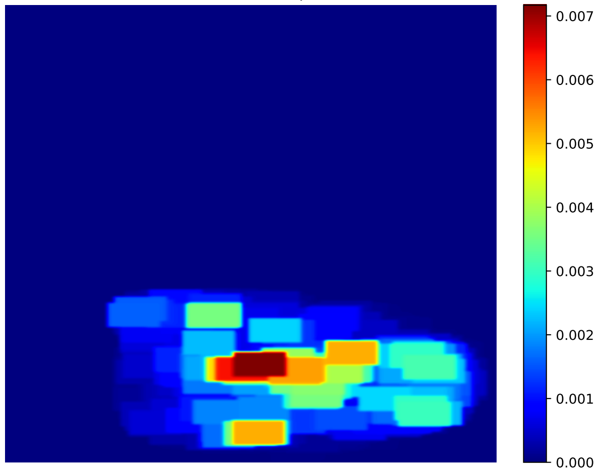
Attention Heatmap - 42
