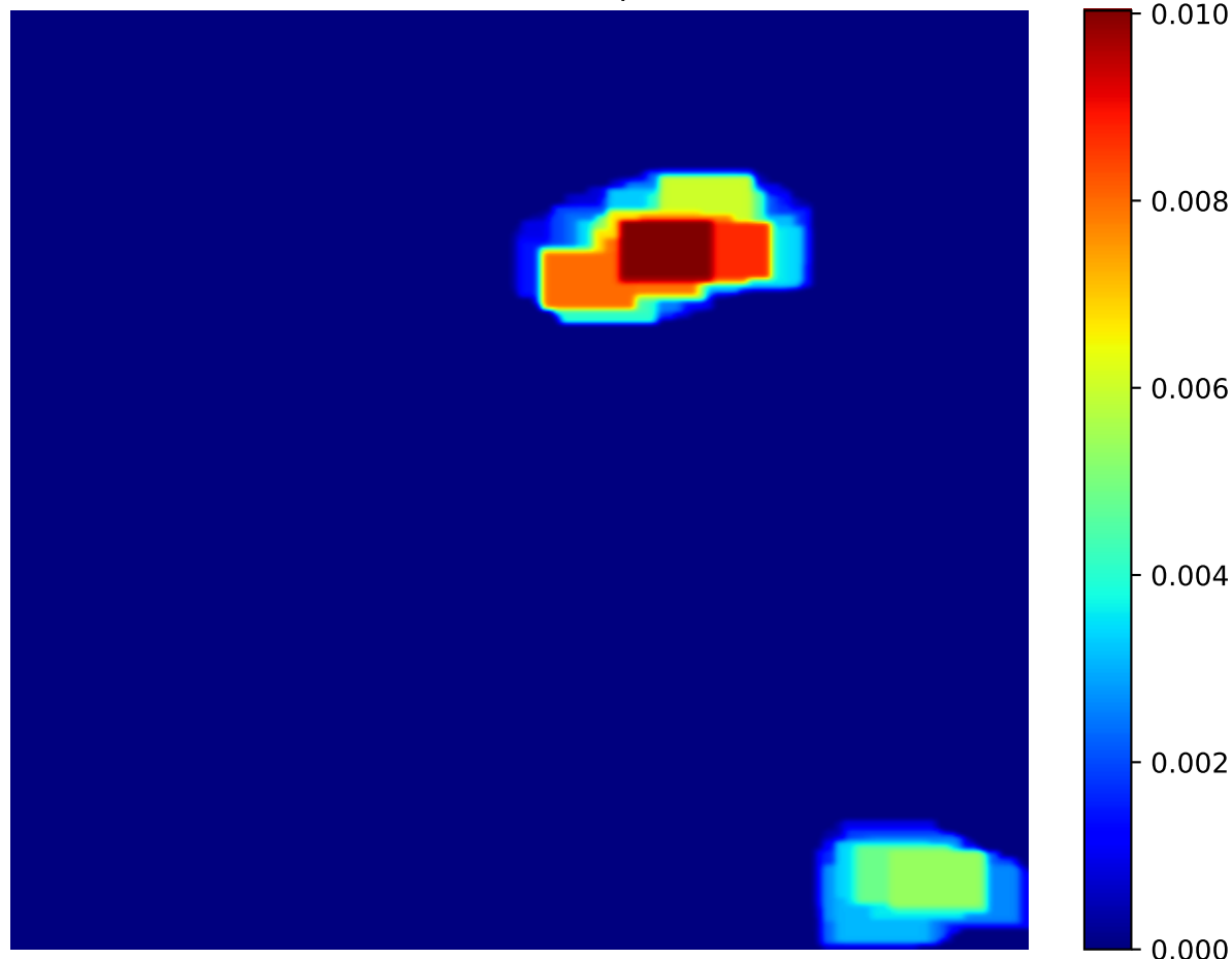
Attention Heatmap - 12
