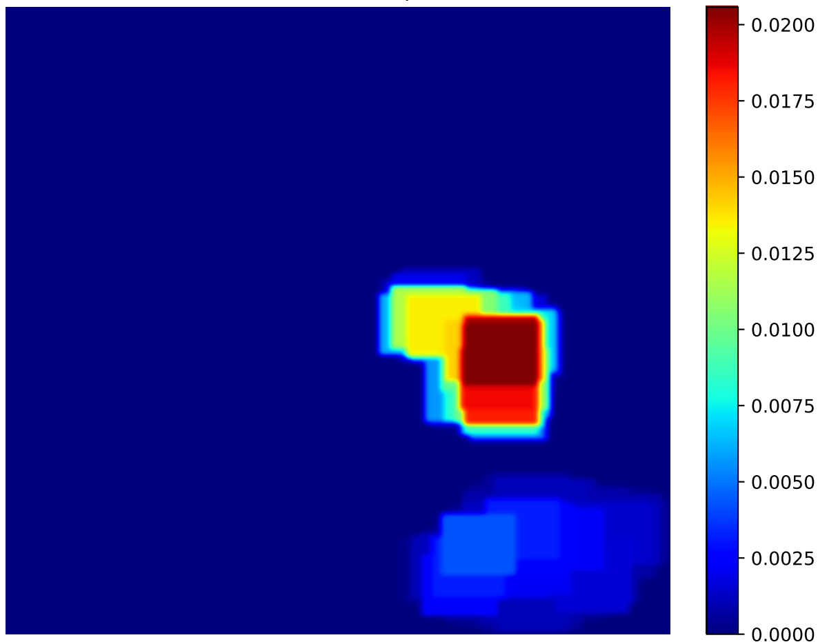
Attention Heatmap - 47
