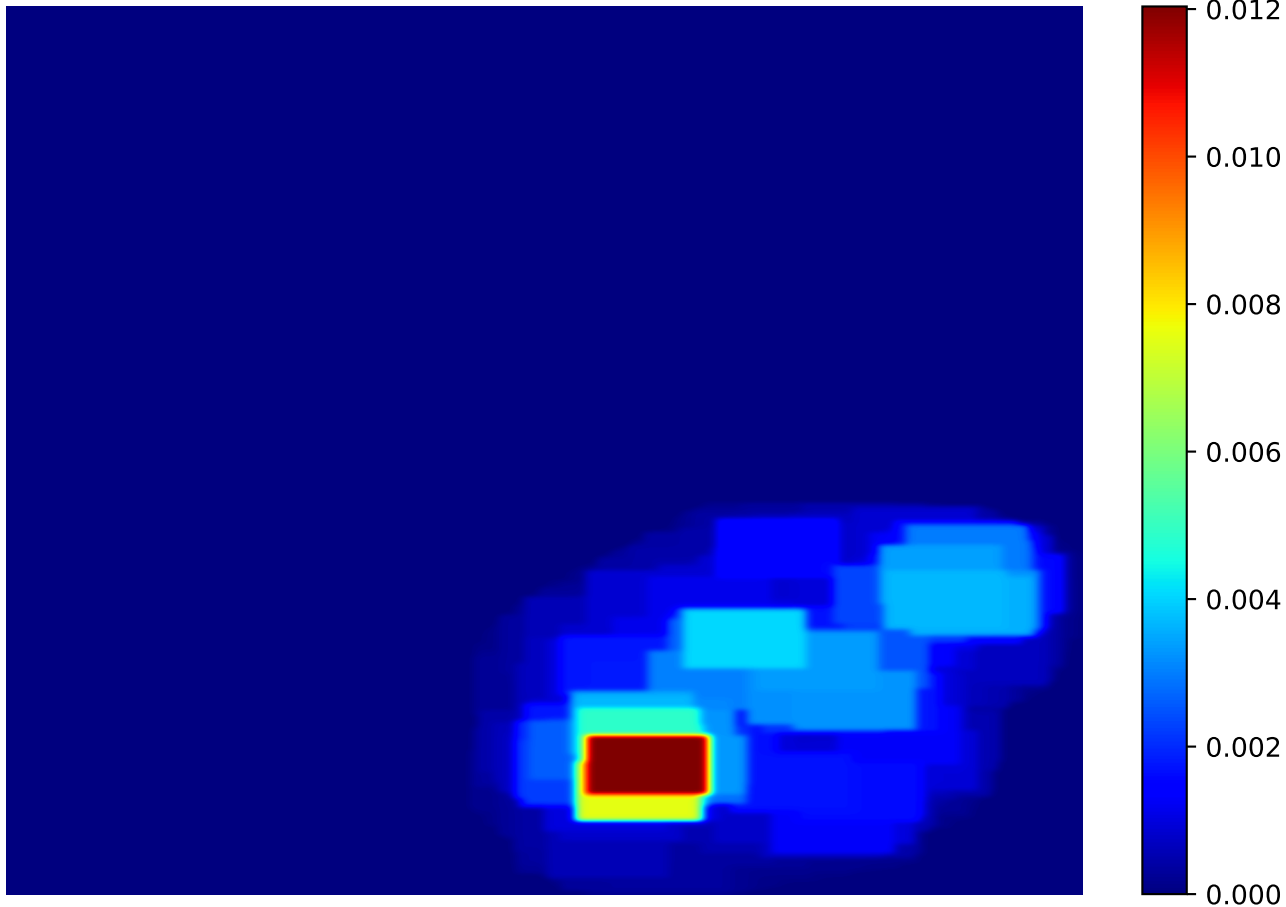
Attention Heatmap - 76 True: Low Risk, Pred: High Risk (prob: 0.760)
