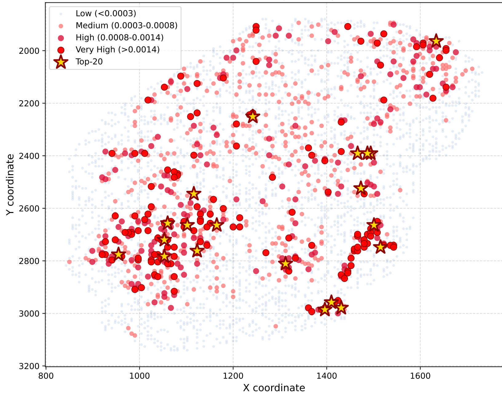
Spatial Distribution of Attention - 76 True: Low Risk, Pred: High Risk (prob: 0.825)
