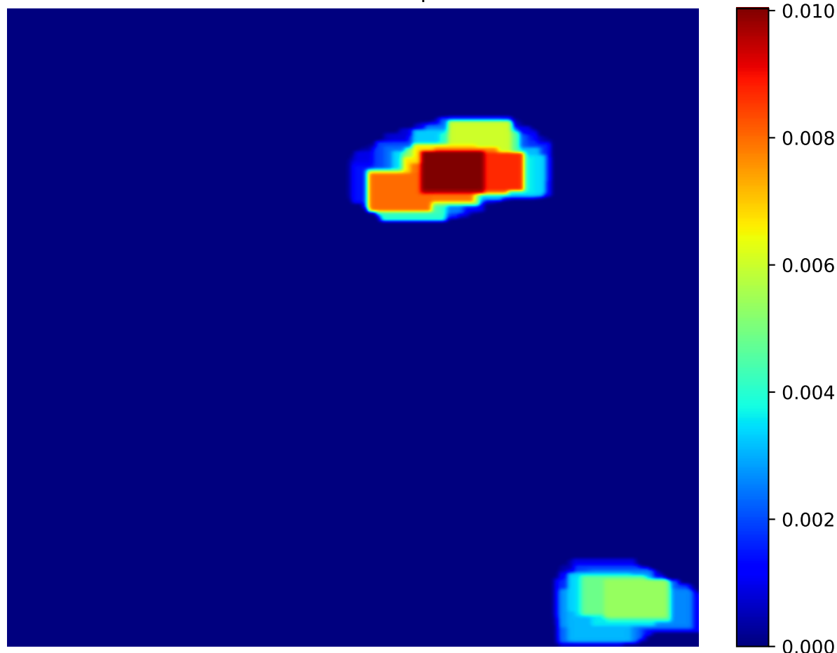
Attention Heatmap - 12
