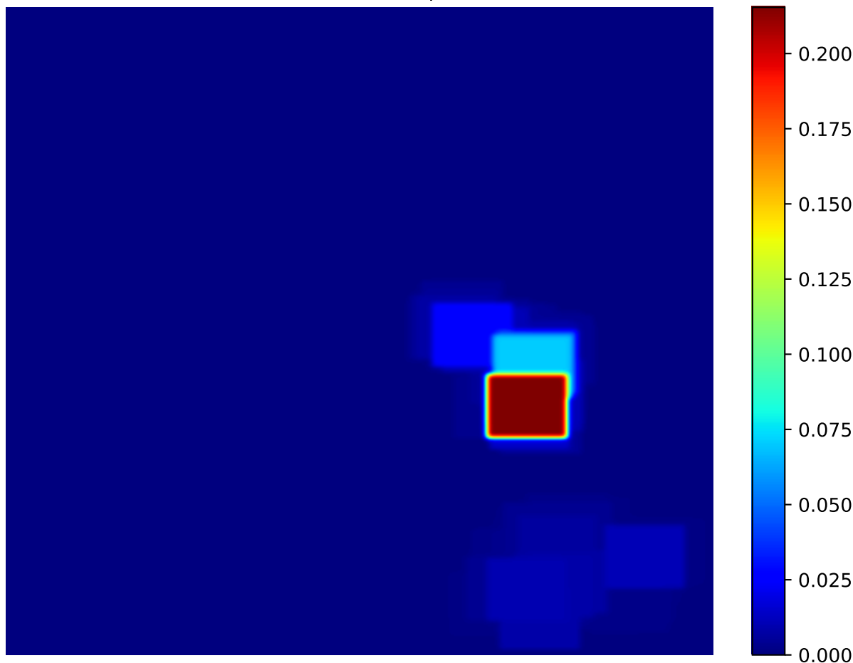
Attention Heatmap - 47
