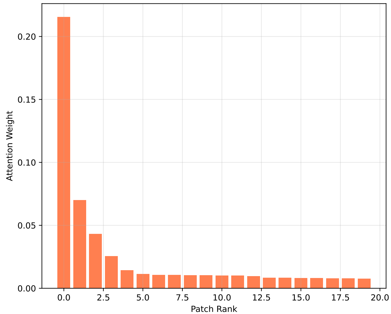
Top-20 Patches Cumulative: 0.507
