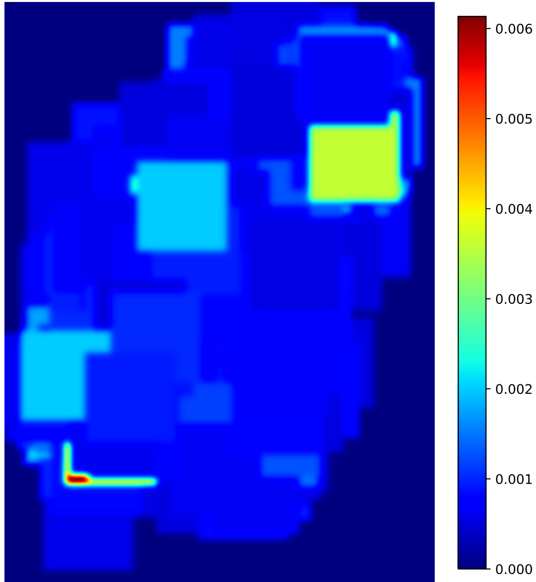
Attention Heatmap
