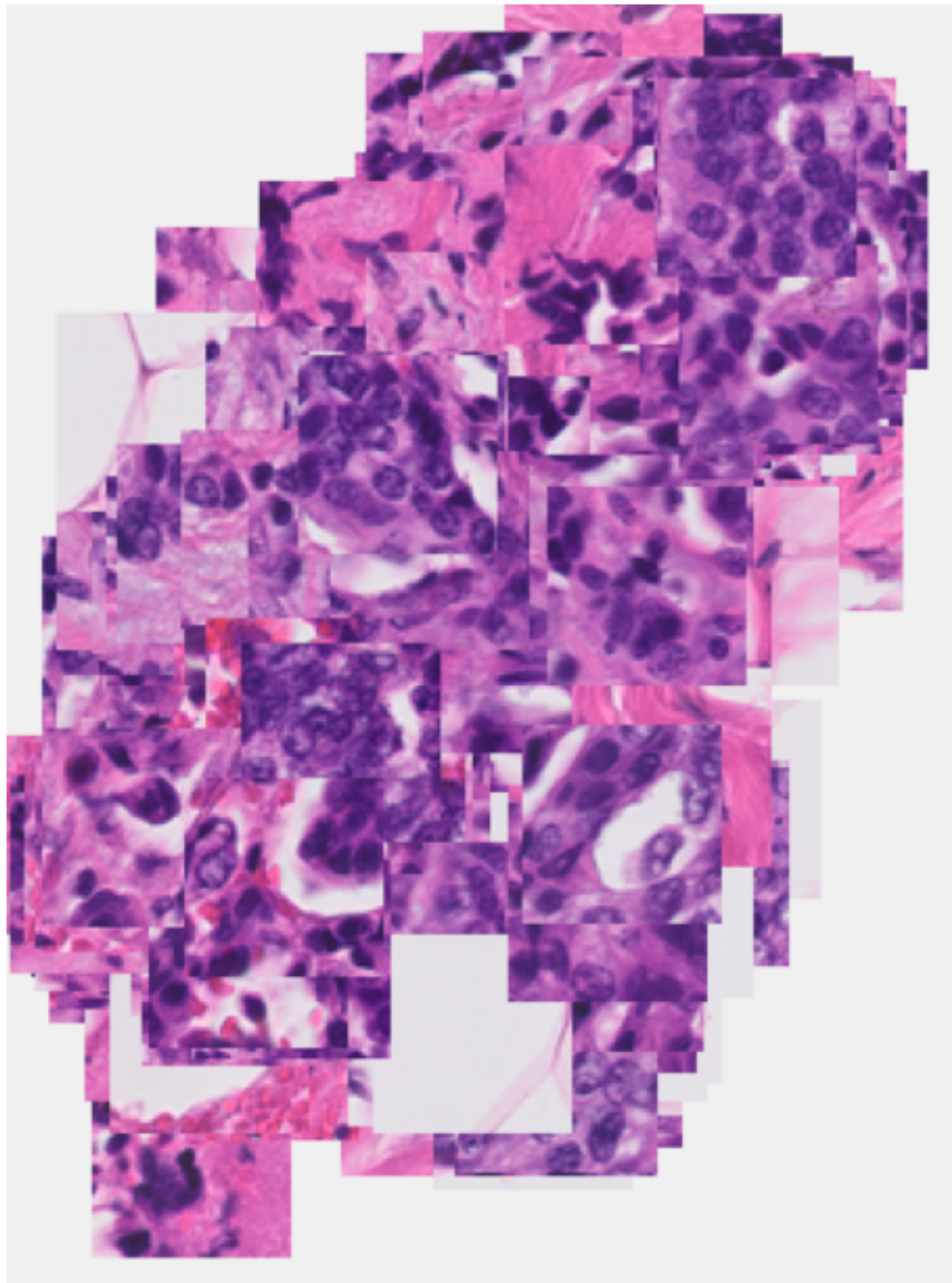
WSI Reconstruction - 76
