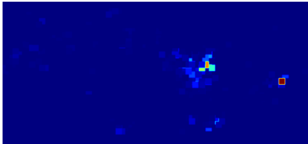
Attention Heatmap
