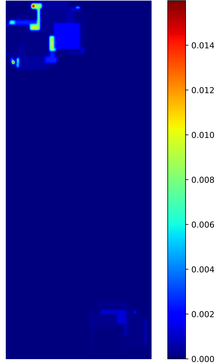
Attention Heatmap
