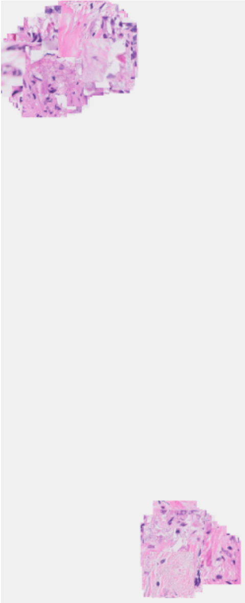
WSI Reconstruction - 12
