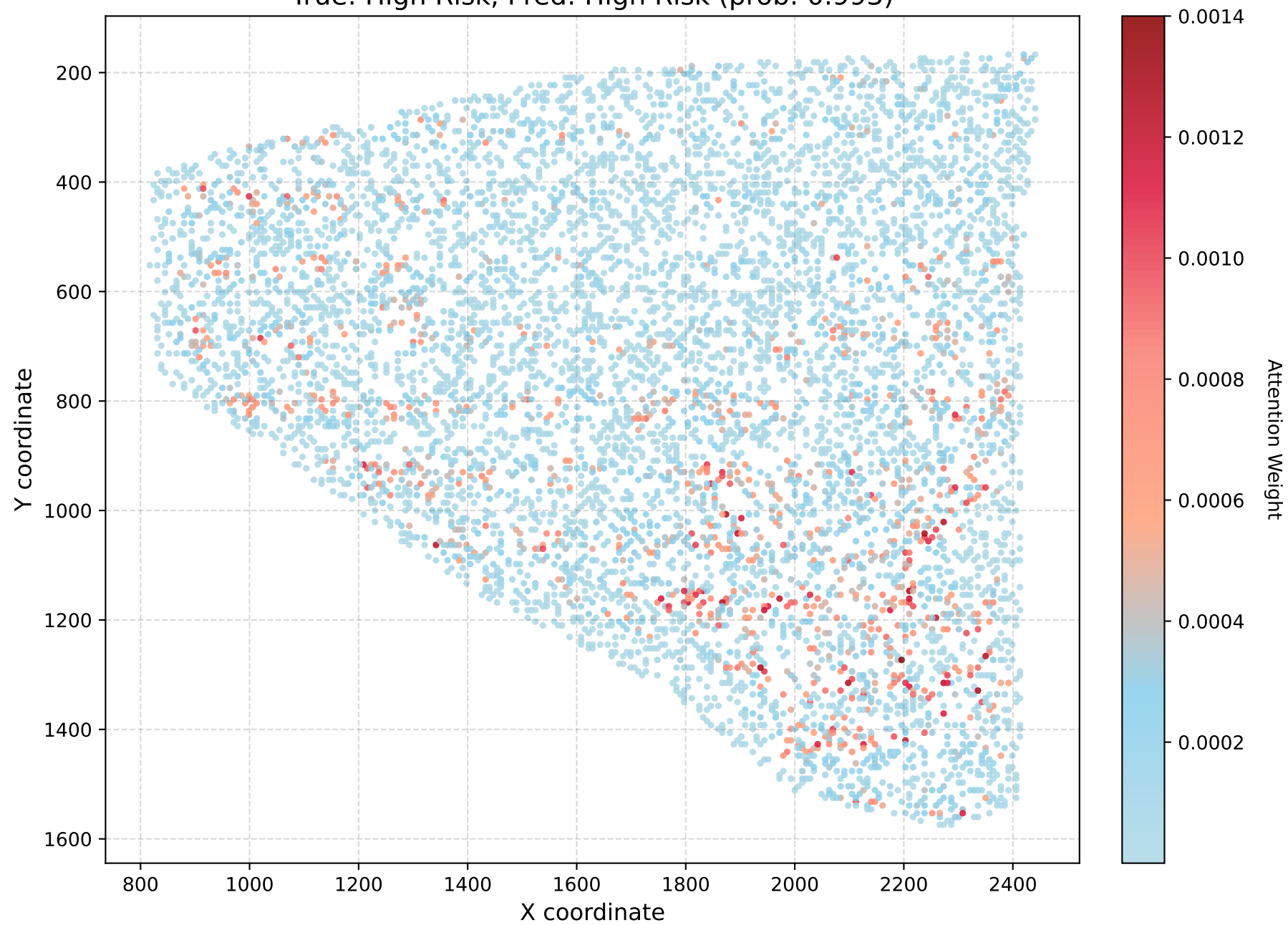
Spatial Distribution of Attention - 63 True: High Risk, Pred: High Risk (prob: 0.993)
