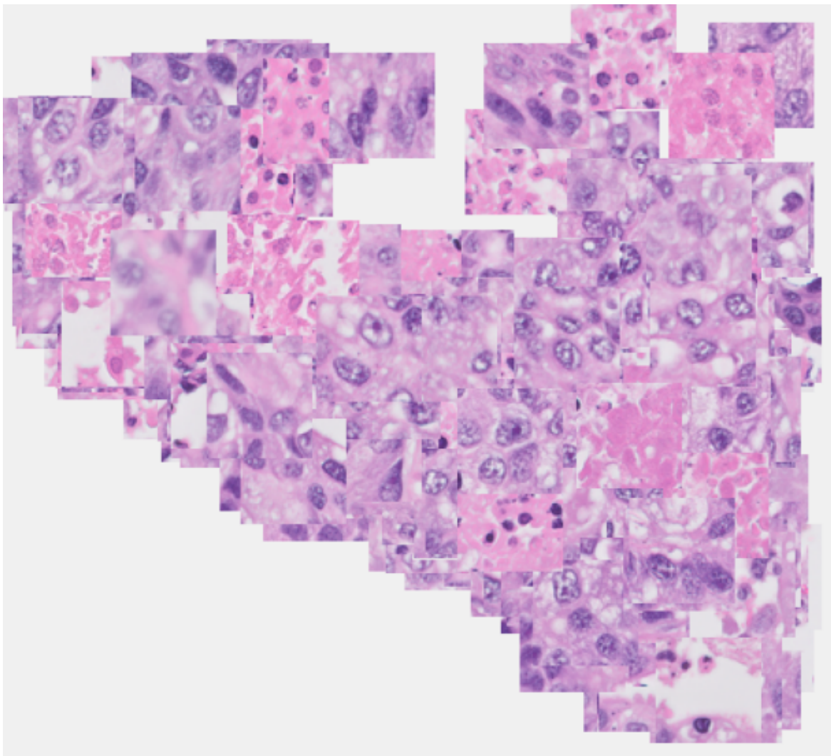
WSI Reconstruction - 63
