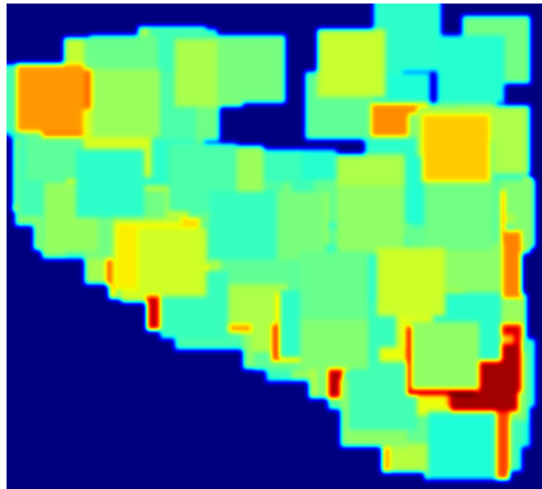
Attention Heatmap
