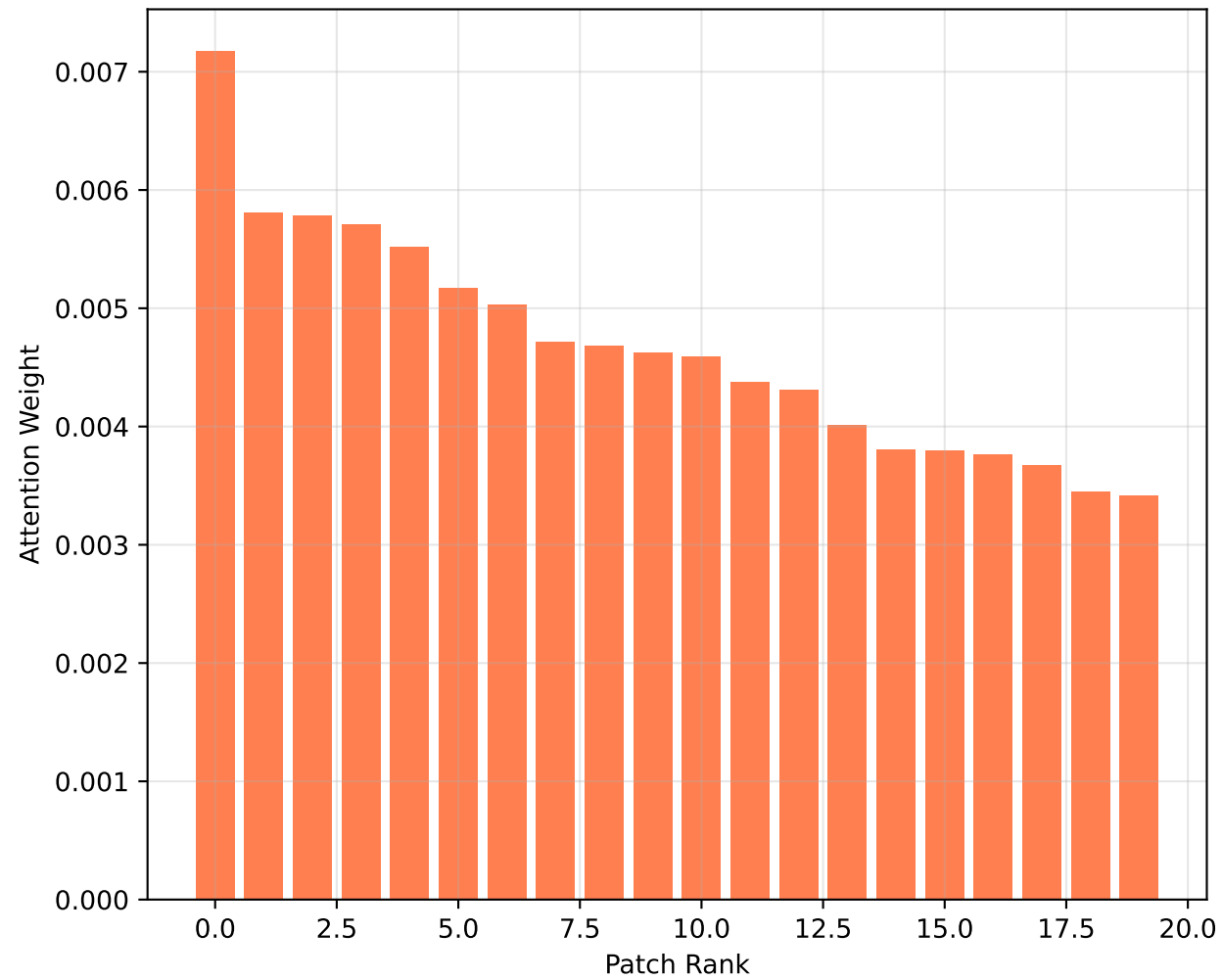
Top-20 Patches Cumulative: 0.093
