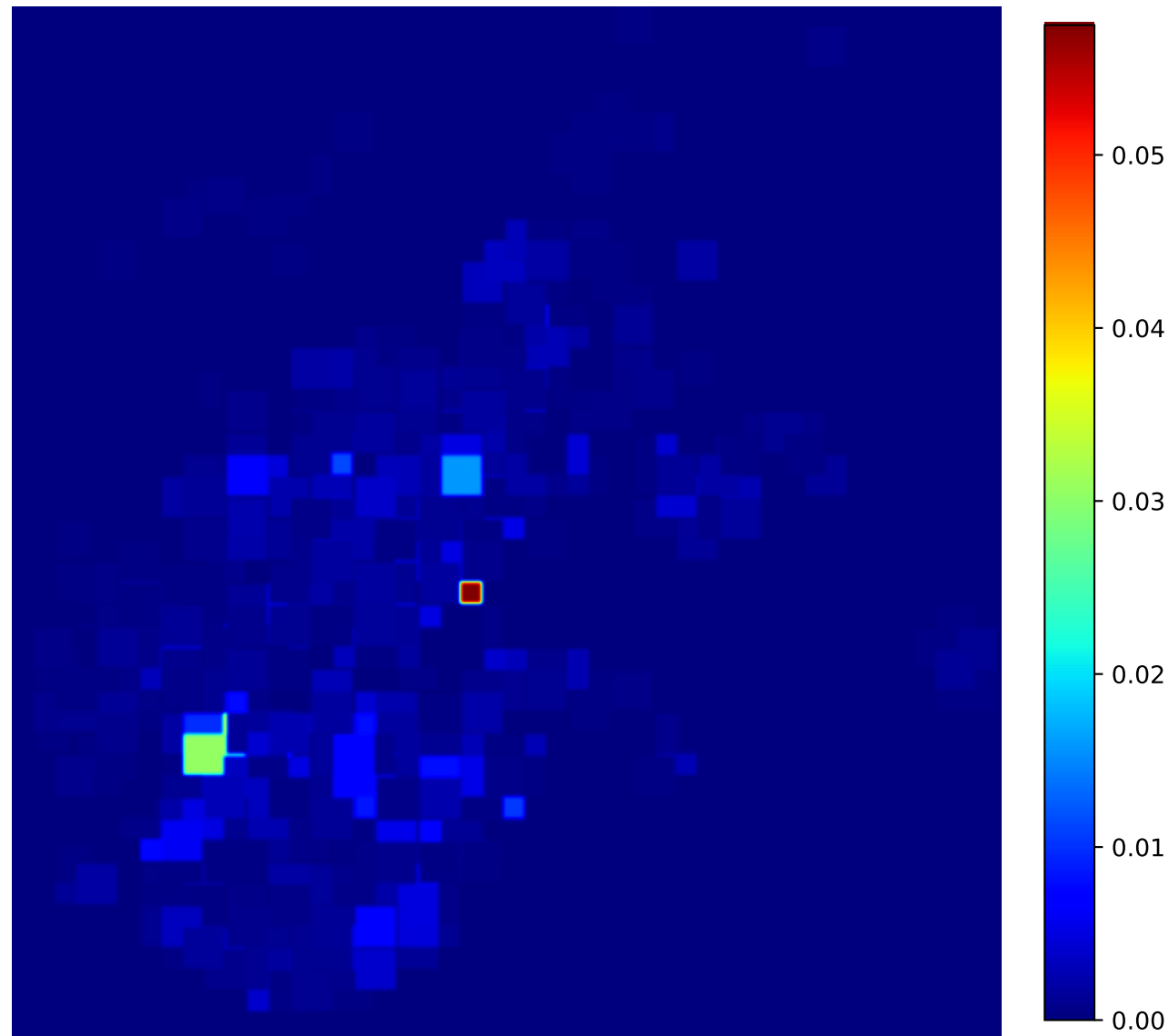
Attention Heatmap
