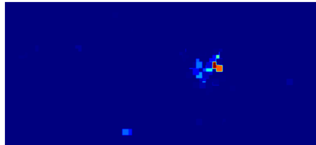
Attention Heatmap
