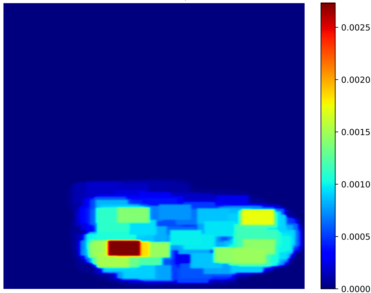
Attention Heatmap - 42
