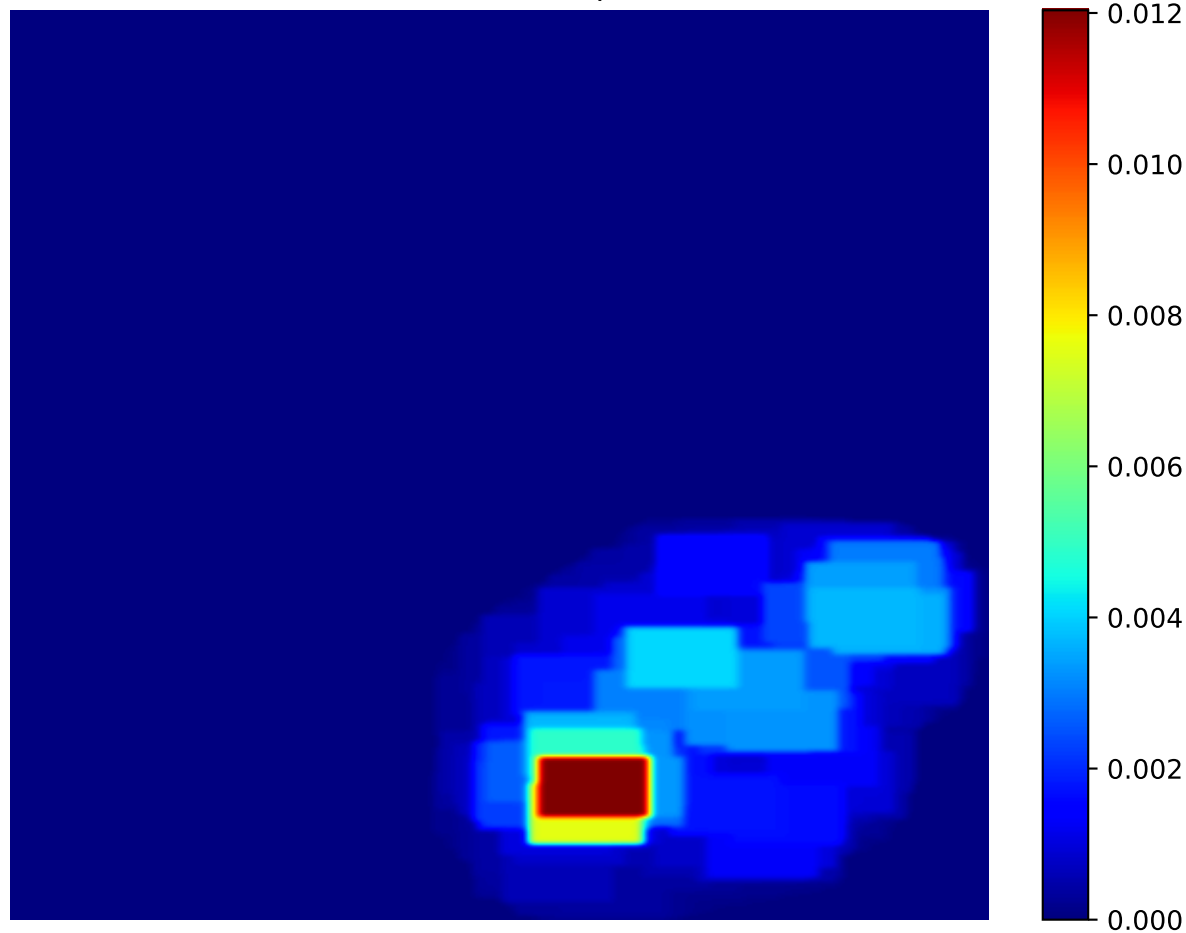
Attention Heatmap - 76
