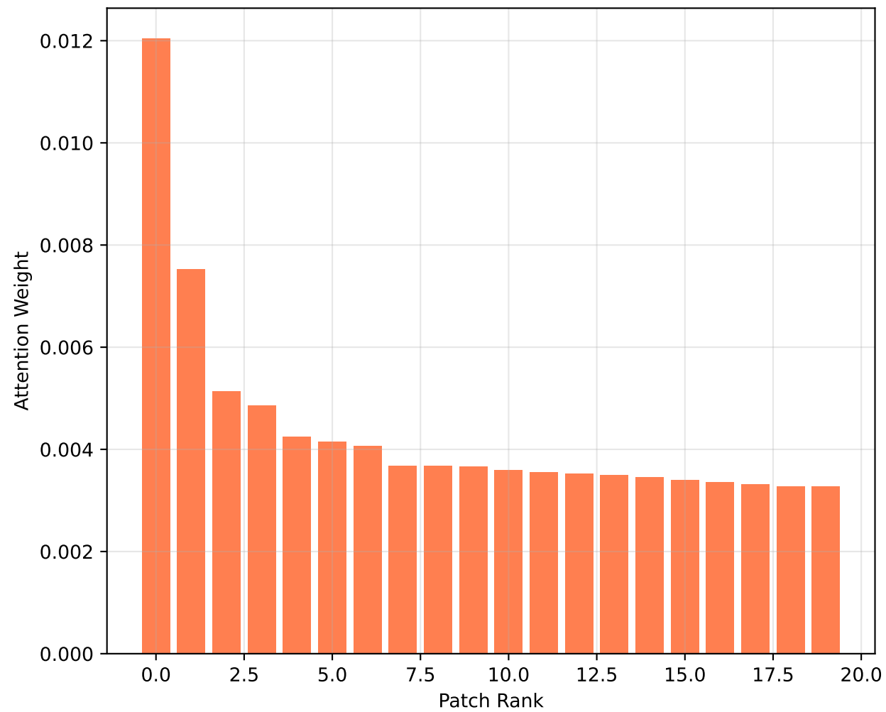
Top-20 Patches Cumulative: 0.087
