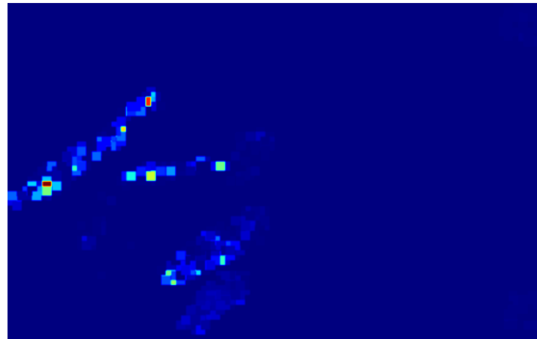
Attention Heatmap
