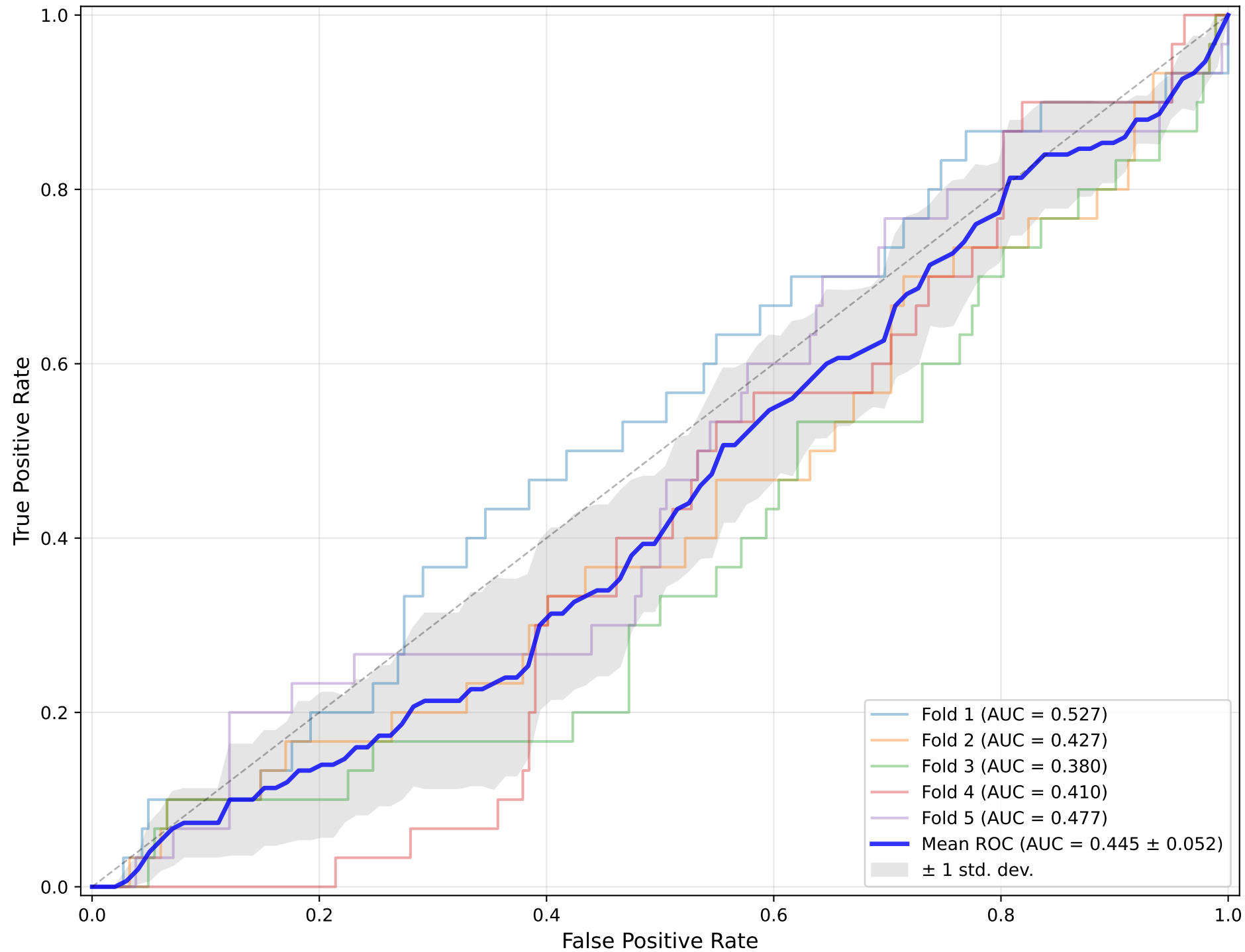
ECU External Validation - ROC Curves
