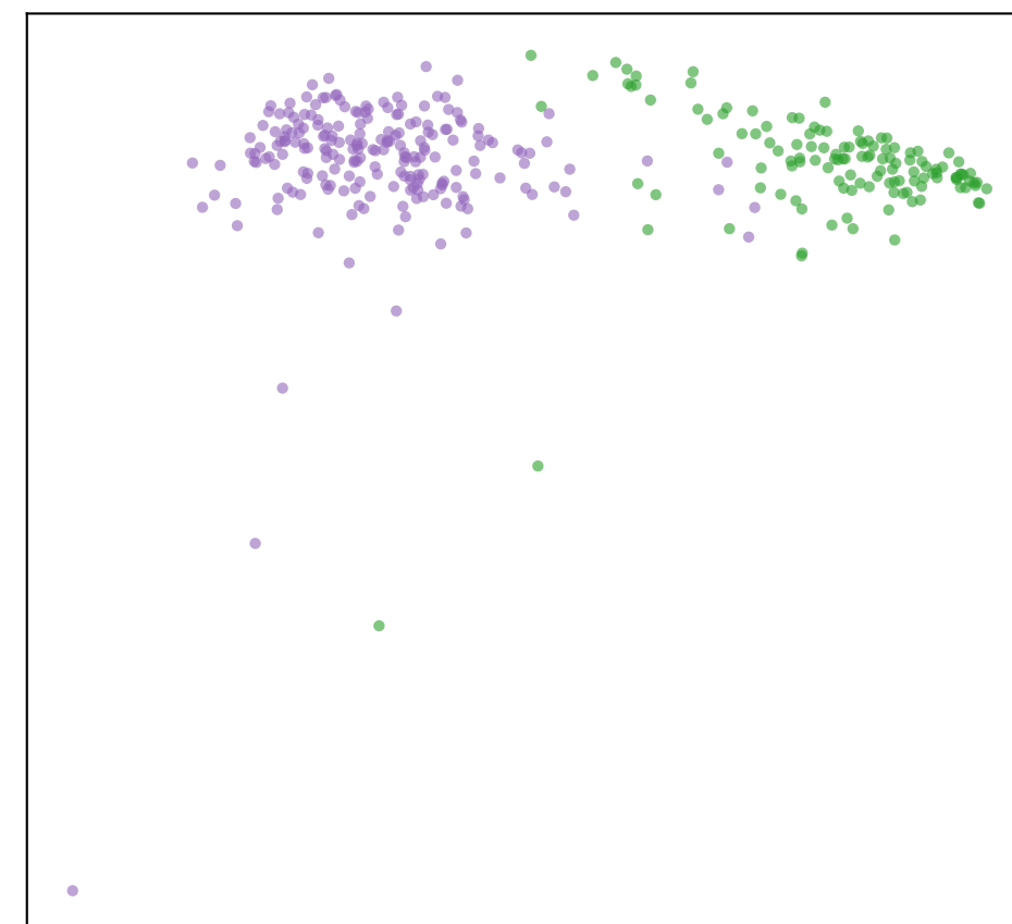
DINOv2 + CLAM
