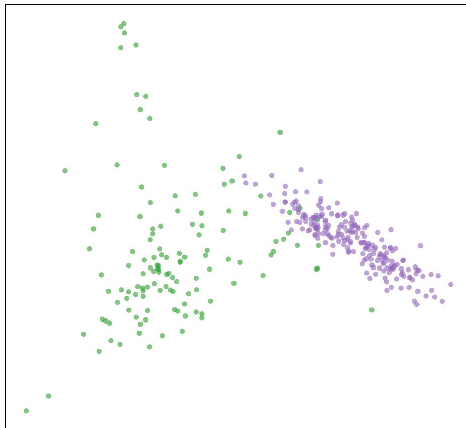
ResNet-18 + CLAM
