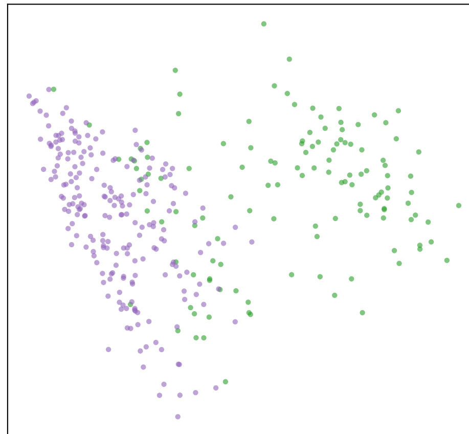
ResNet-50 + ACMIL
