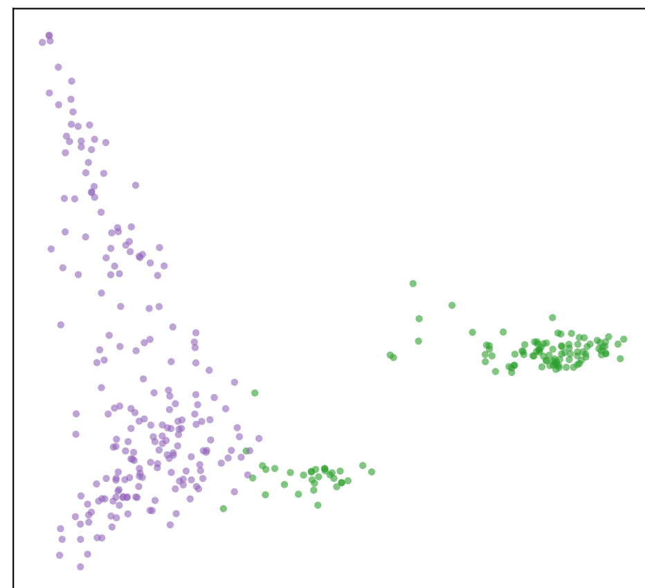
UNI2-H + ABMIL
