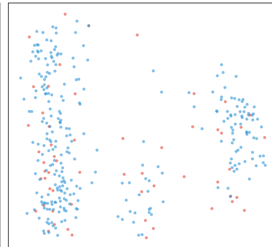
DINOv2 + CLAM
