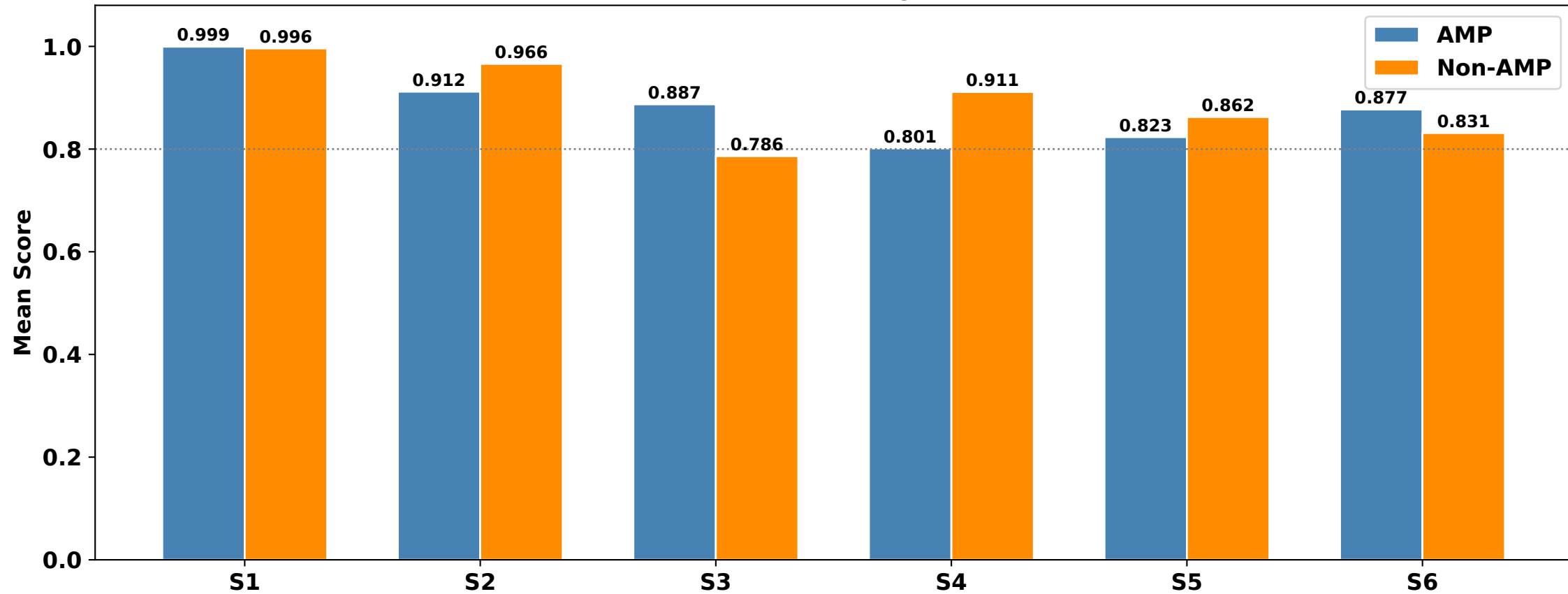
Per-Statement Mean Plausibility Scores (Qwen2.5:7b)
