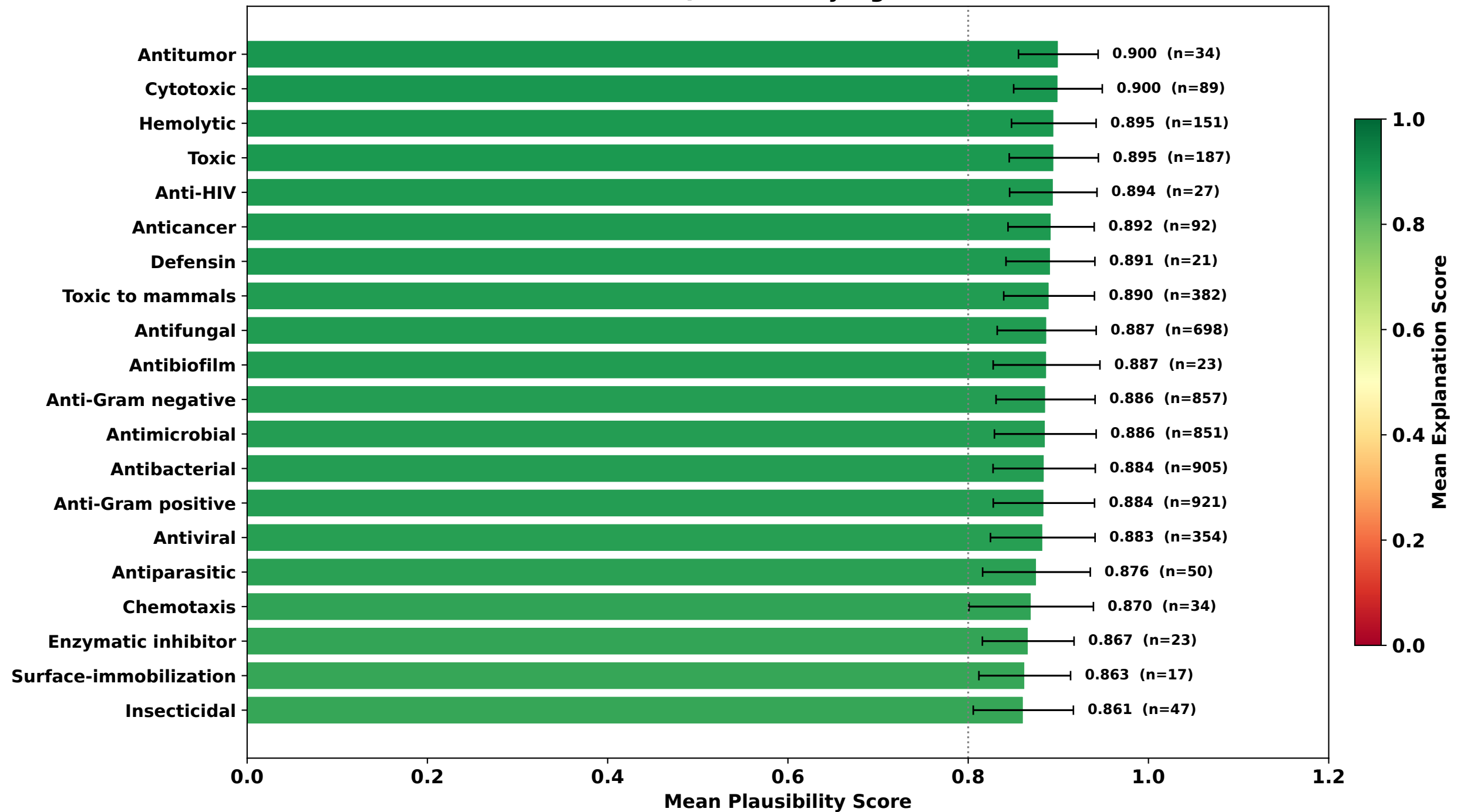
Mean Explanation Score by AMP Activity (Qwen2.5:7b judge)
