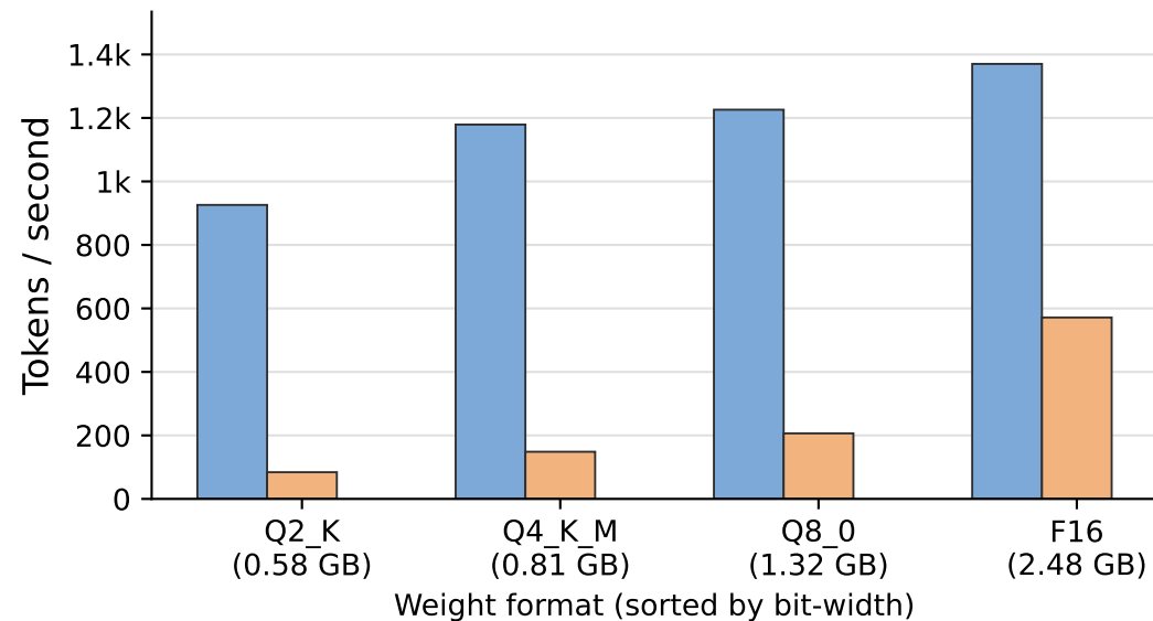
Decode — depth 0
