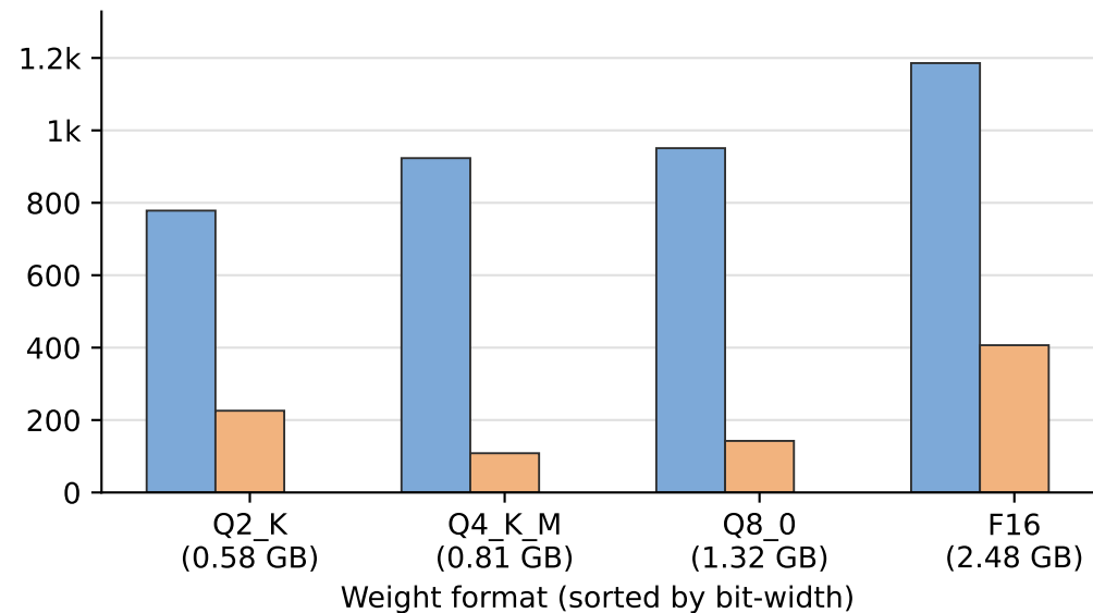
Decode — depth 2048
