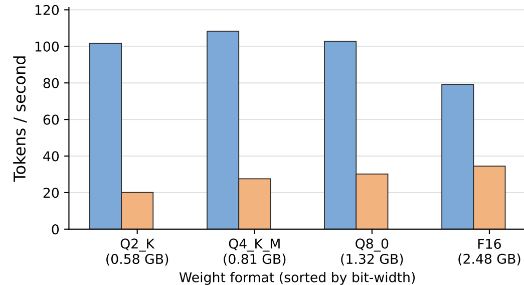
Decode — depth 0
