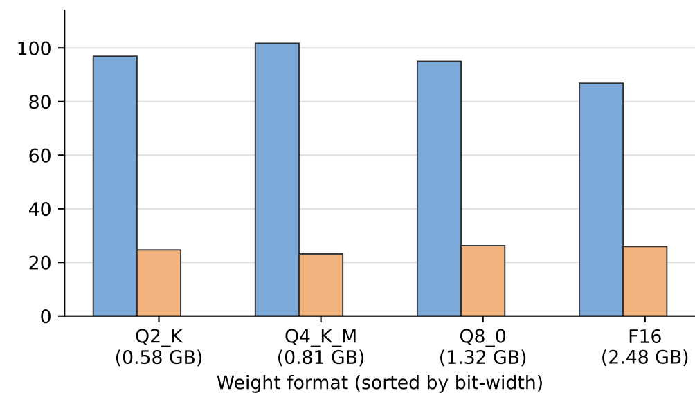
Decode — depth 2048
