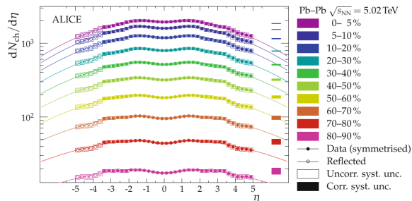
Fig. 5.14 ALICE result of mid-rapidity dN_{ch}/d\eta for Pb+Pb collisions at \sqrt{s_{NN}} = 5.02 TeV. Reprinted under CC-BY-4.0 license from [7]. ©2017, ALICE Collaboration
