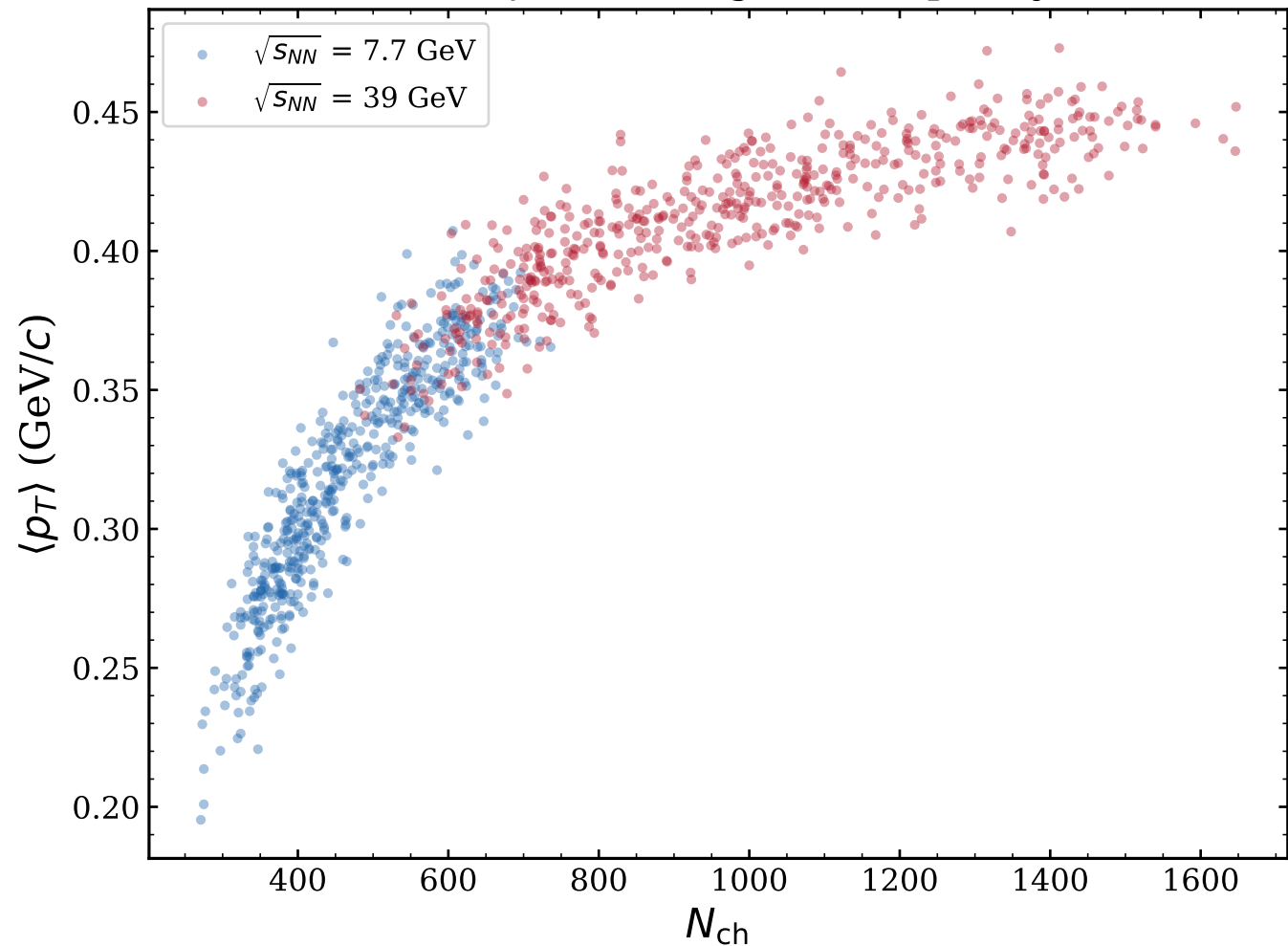
Mean p_T vs Charged Multiplicity
