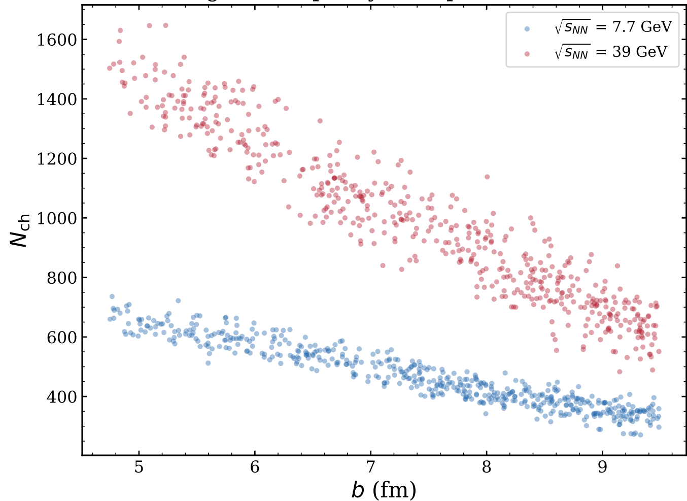
Charged Multiplicity vs Impact Parameter
