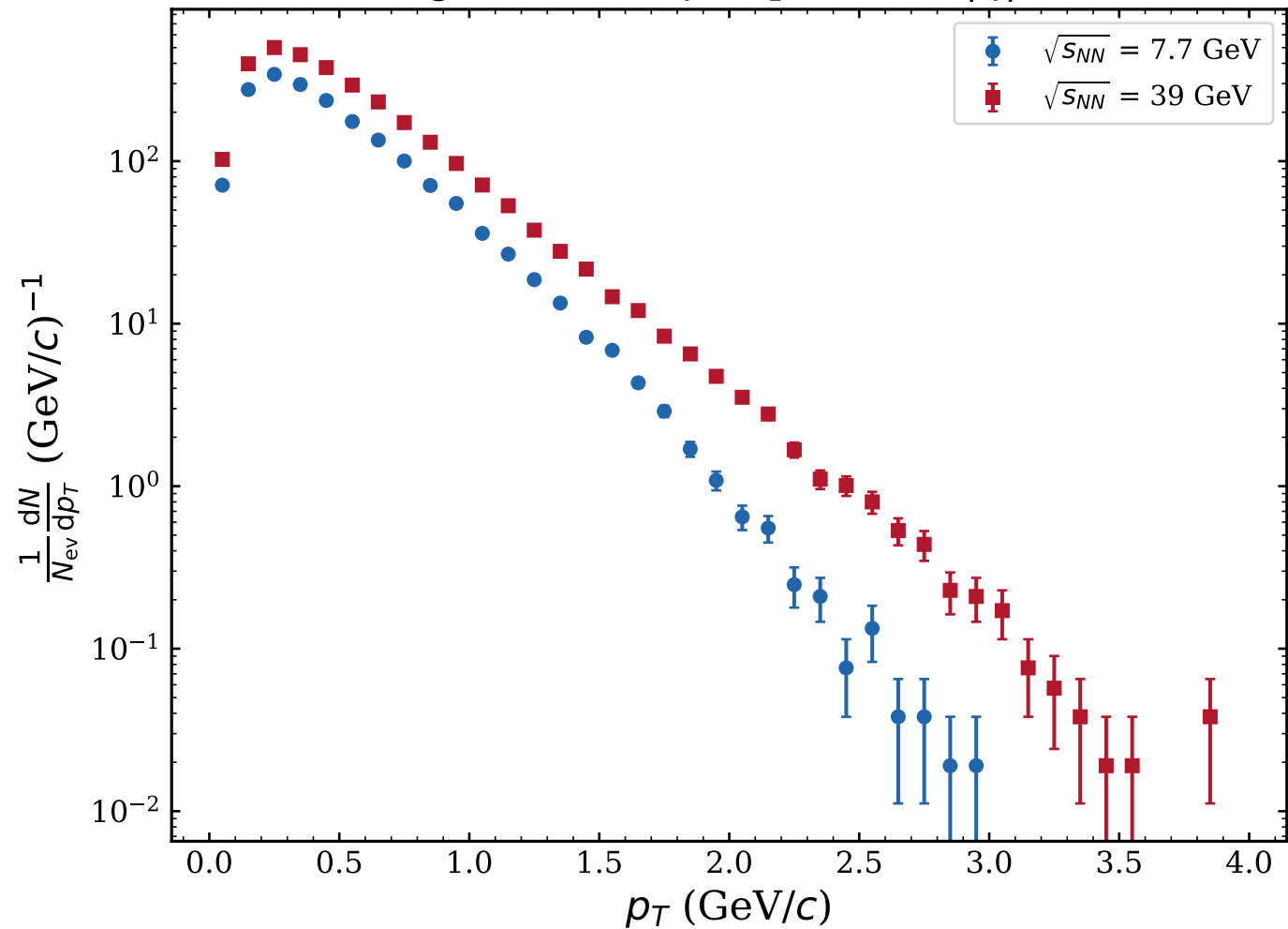
Charged Particle p_T Spectrum, |\eta| < 1.0
